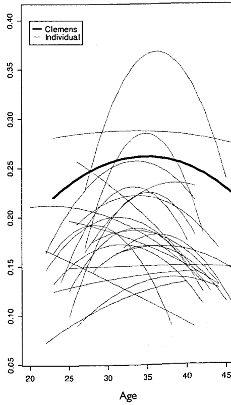
Subset of K rate Career Trajectories
