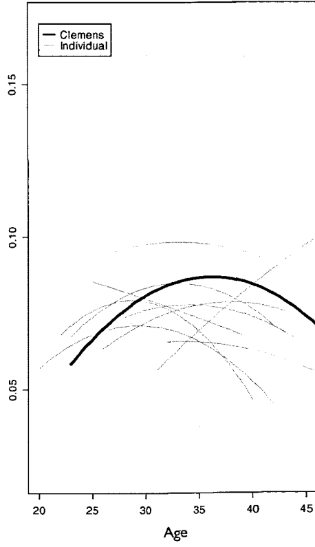
Subset of BB rate Career Trajectories
